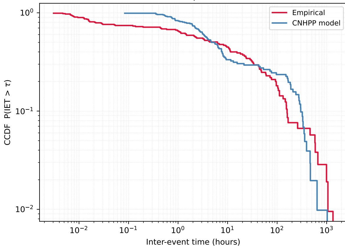
User 1134520908 - Empirical vs CNHPP model
